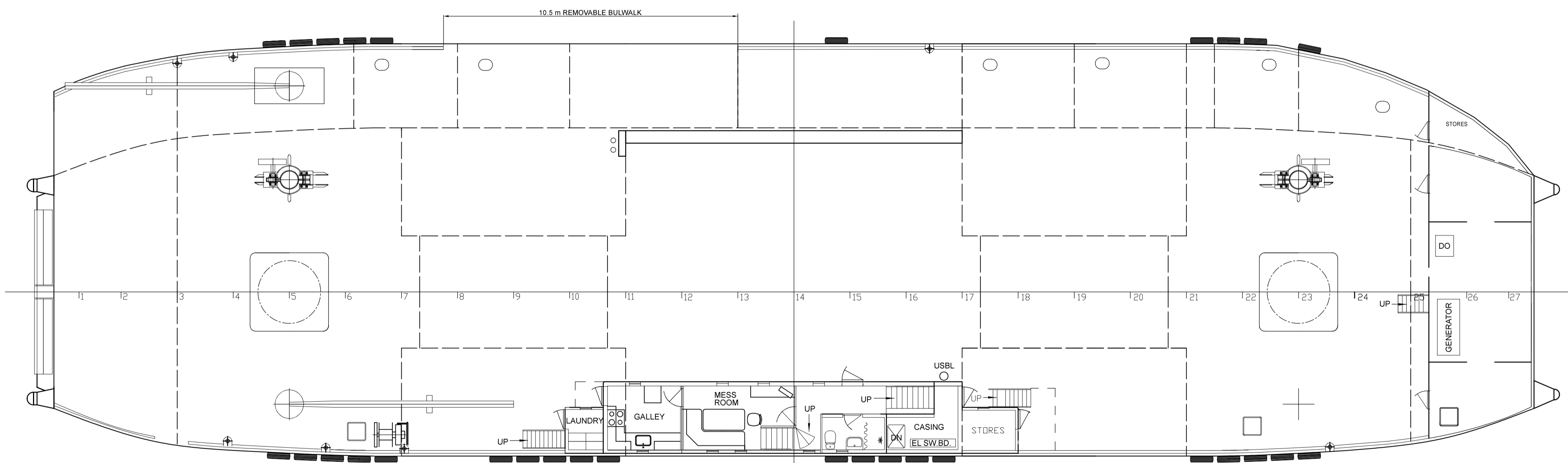
MAIN DECK
